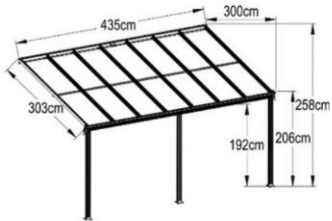
Kingston Lean-To Carport Patio Cover 10' x 14'
